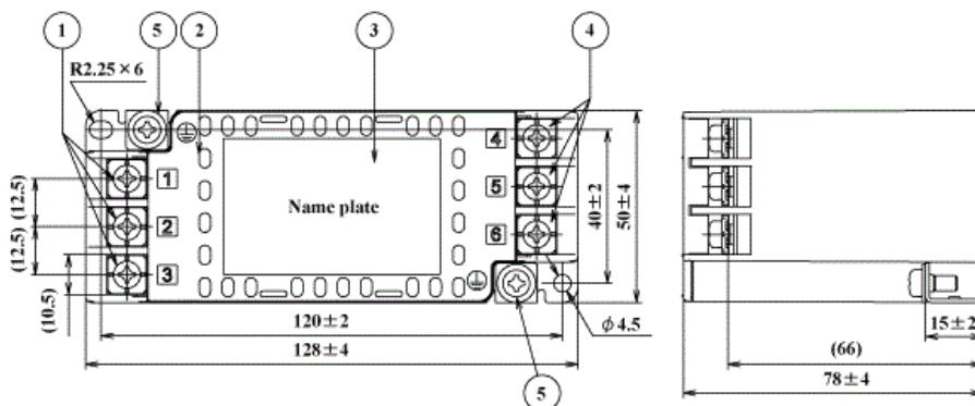
fig.1 (10-30A)
