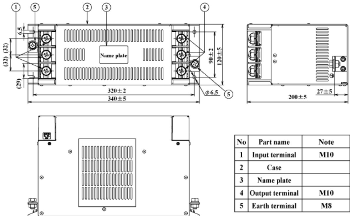
fig.5 (200-300A)
