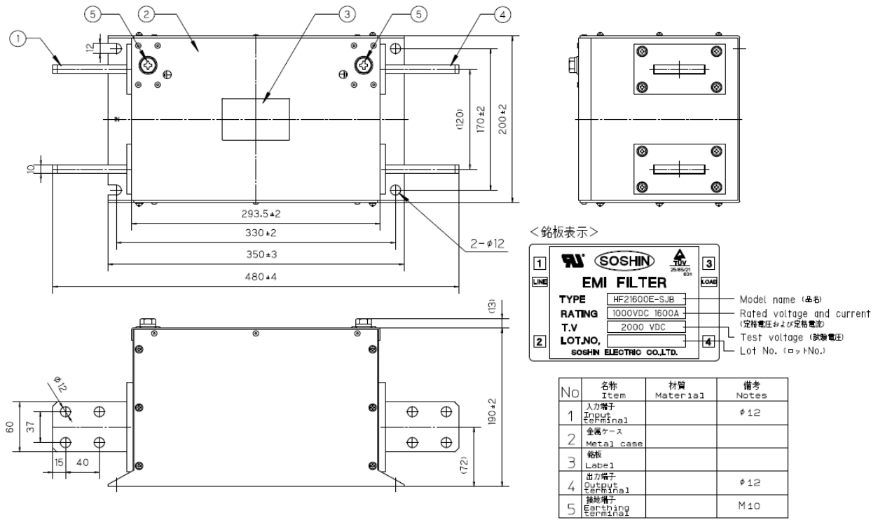
fig.4 (1600A)
