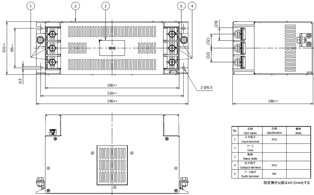
fig. 4 (200A~300A)
