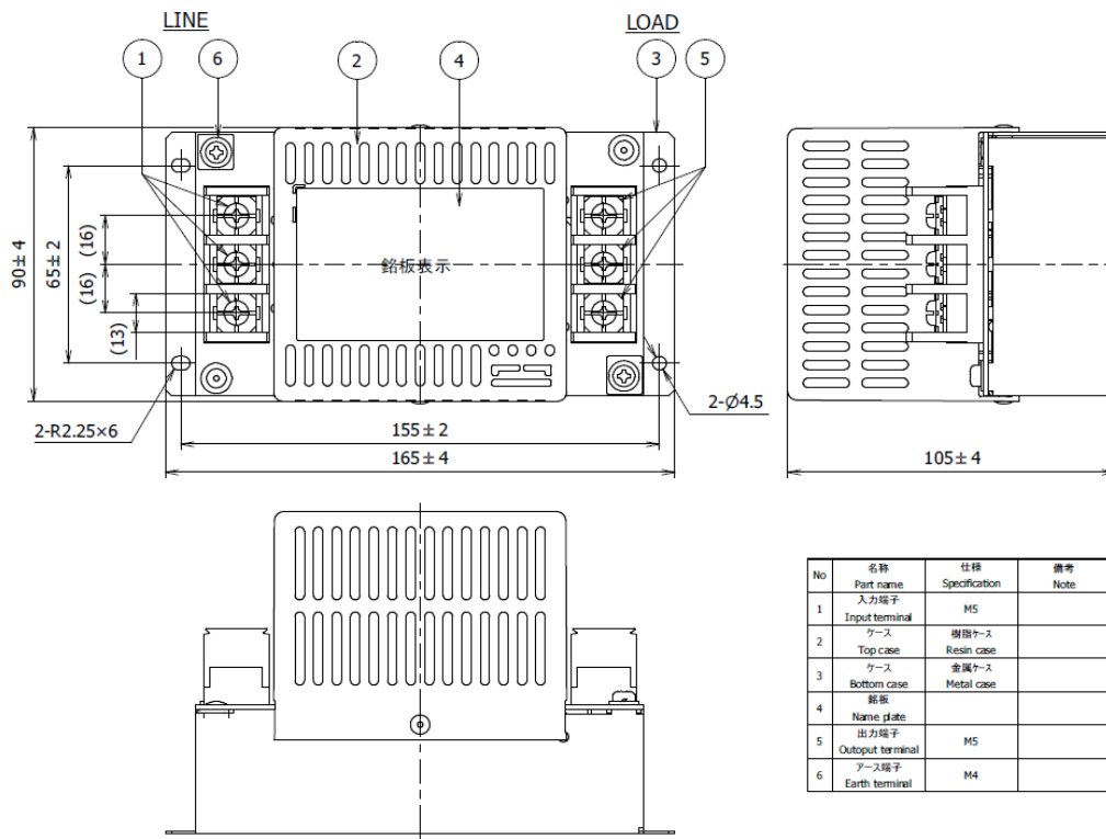
fig.2 (80A, 100A)
