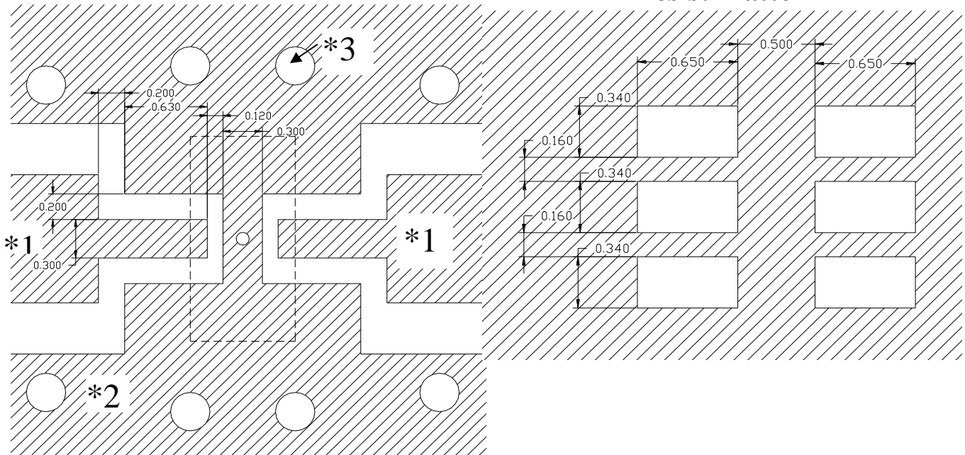
*Land Pattern
