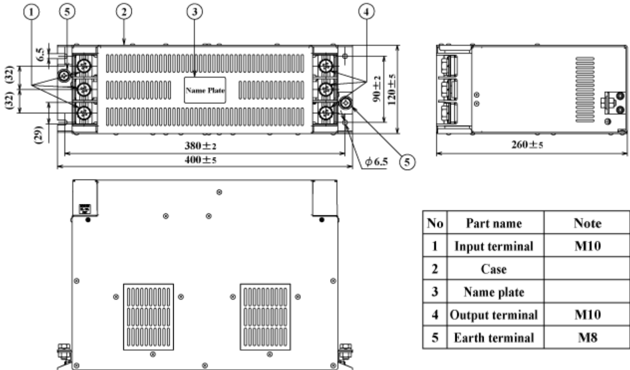
fig.5 (200-300A)
