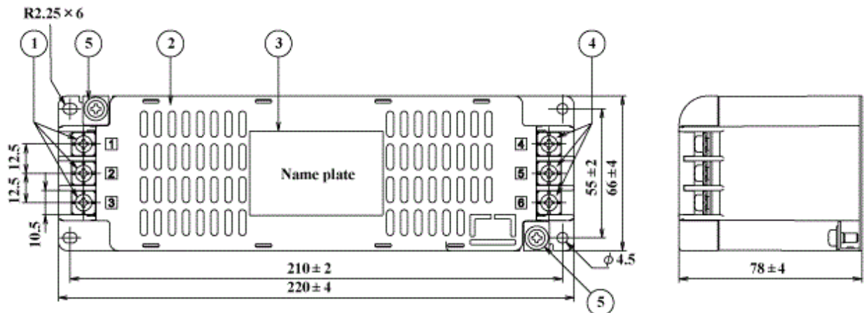
fig.1 (10-30A)
