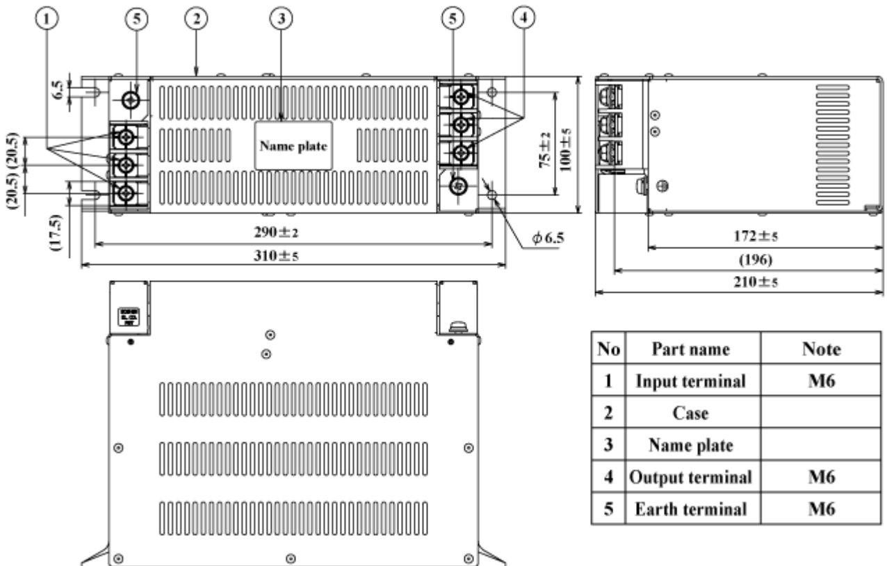
fig.3 (80A, 100A)
