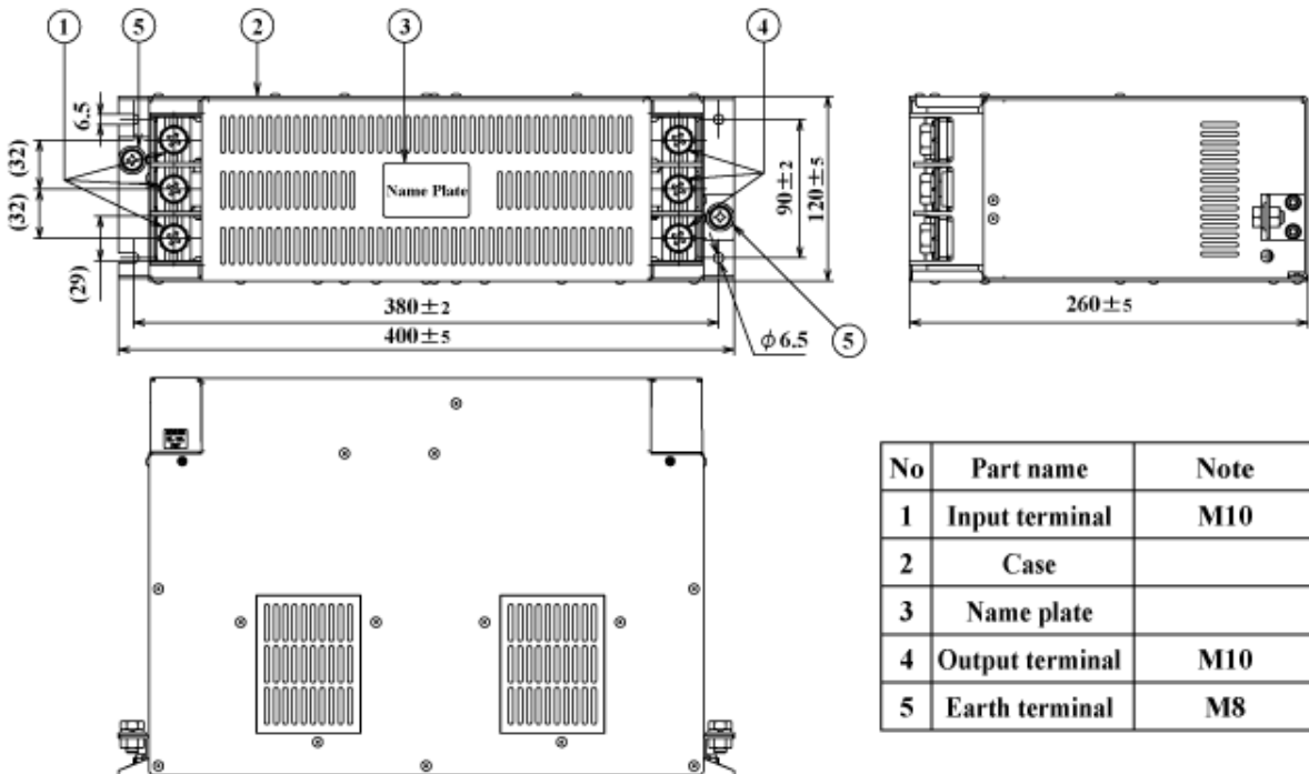
fig.5 (200-300A)
