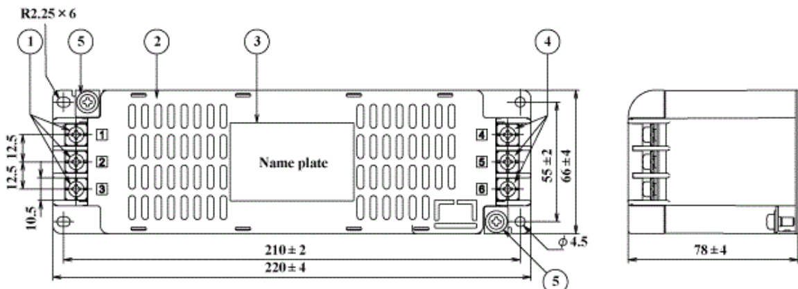
fig.1 (10-30A)
