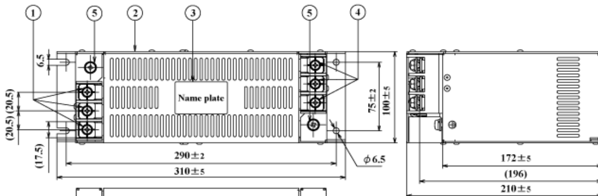
fig.3 (80A, 100A)
