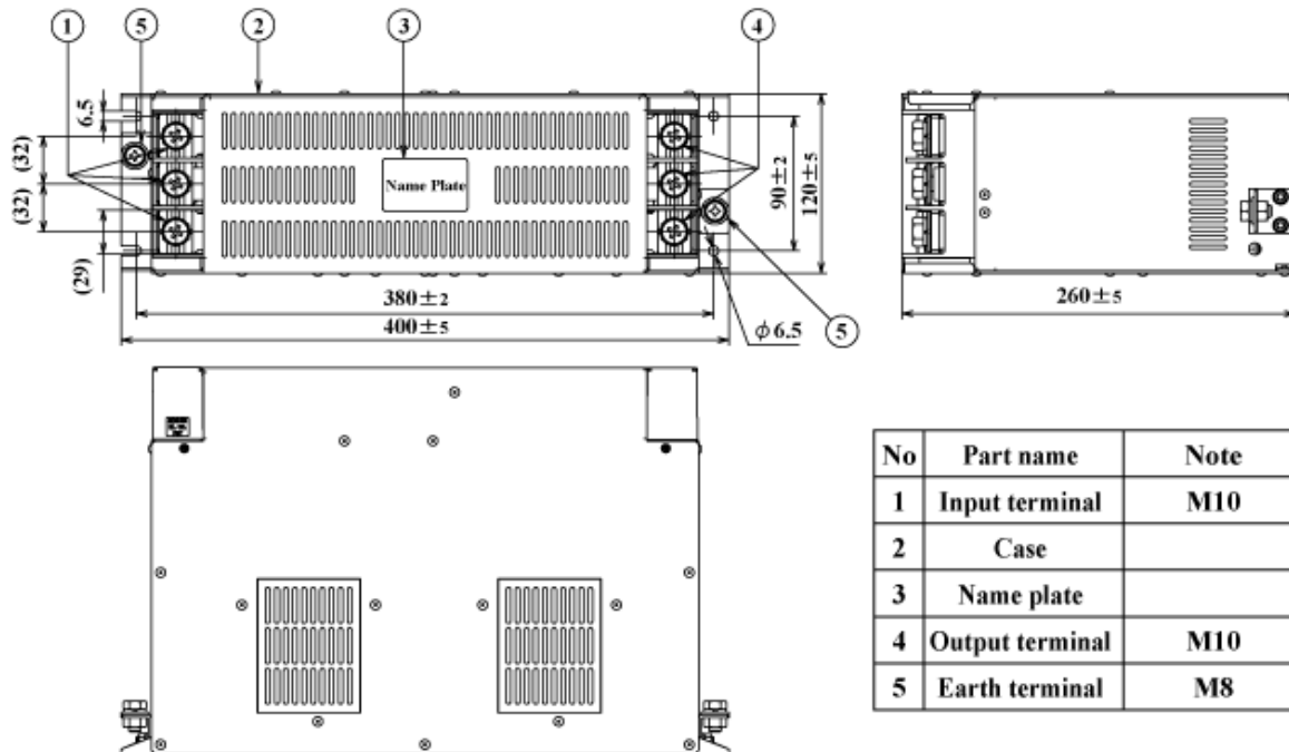
fig.5 (200-300A)
