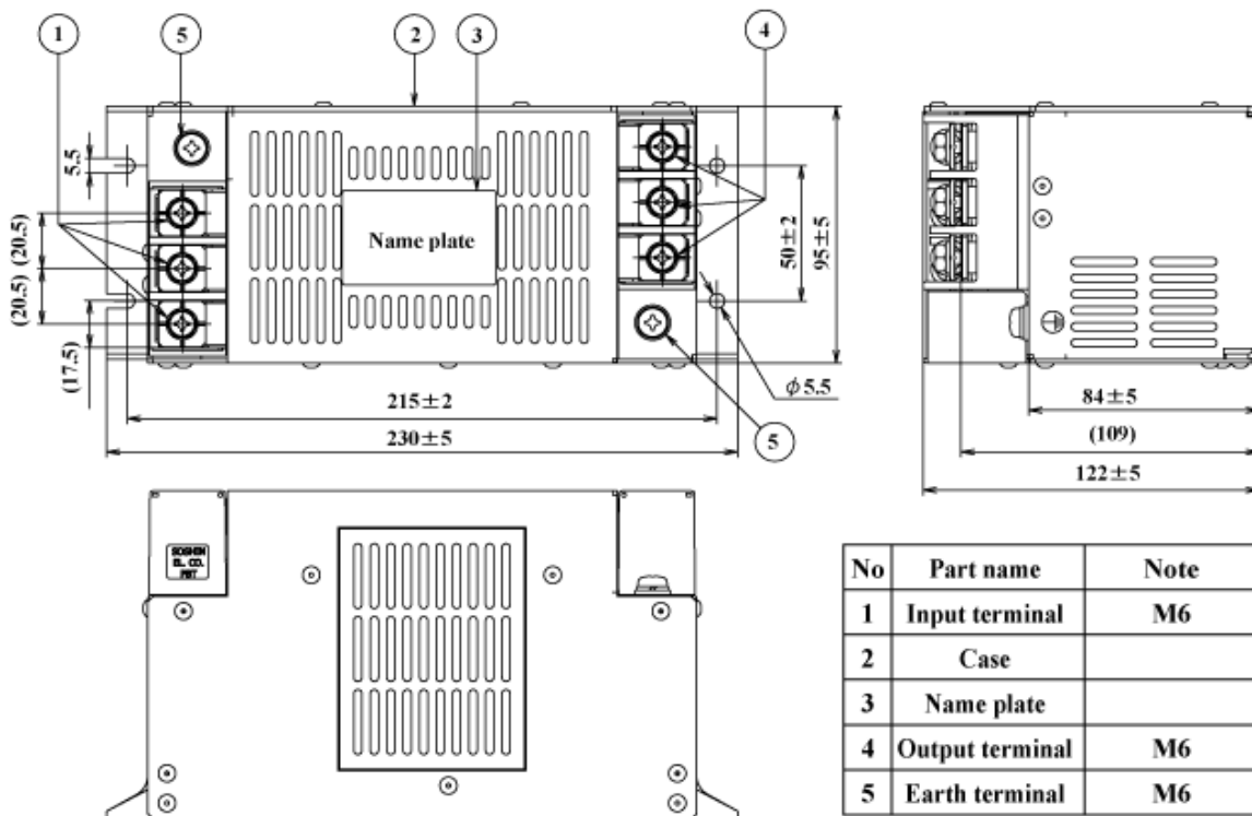
fig.3 (80A, 100A)
