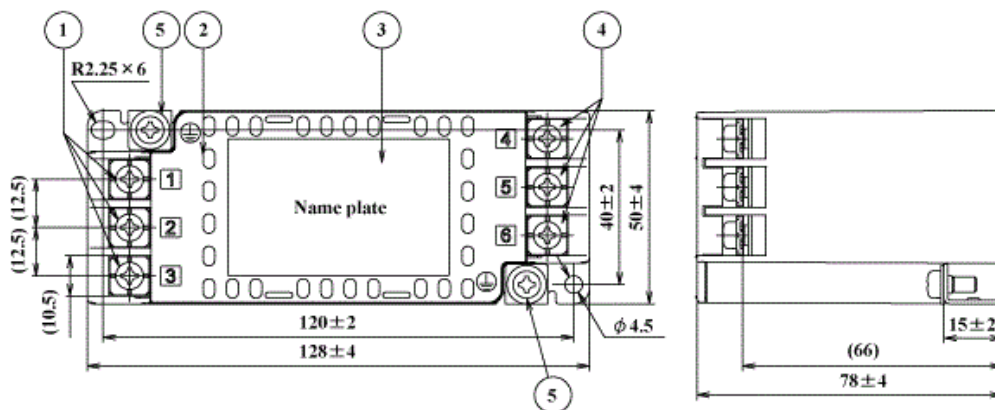
fig.1 (10-30A)
