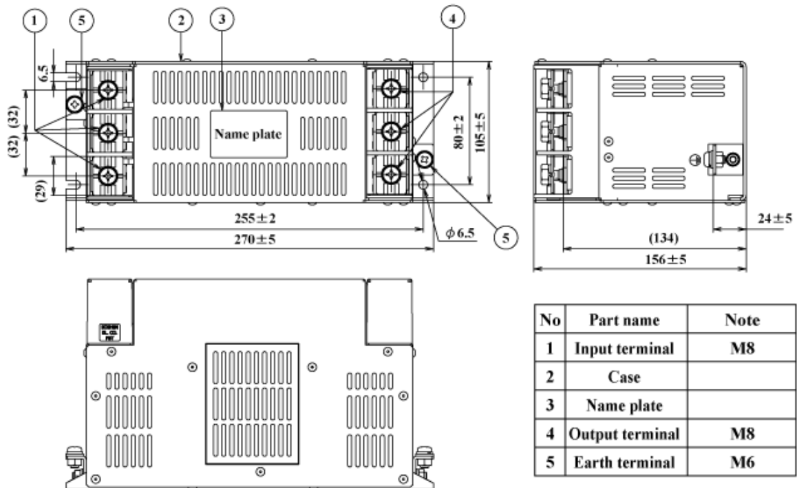
fig.4 (150A, 180A)
