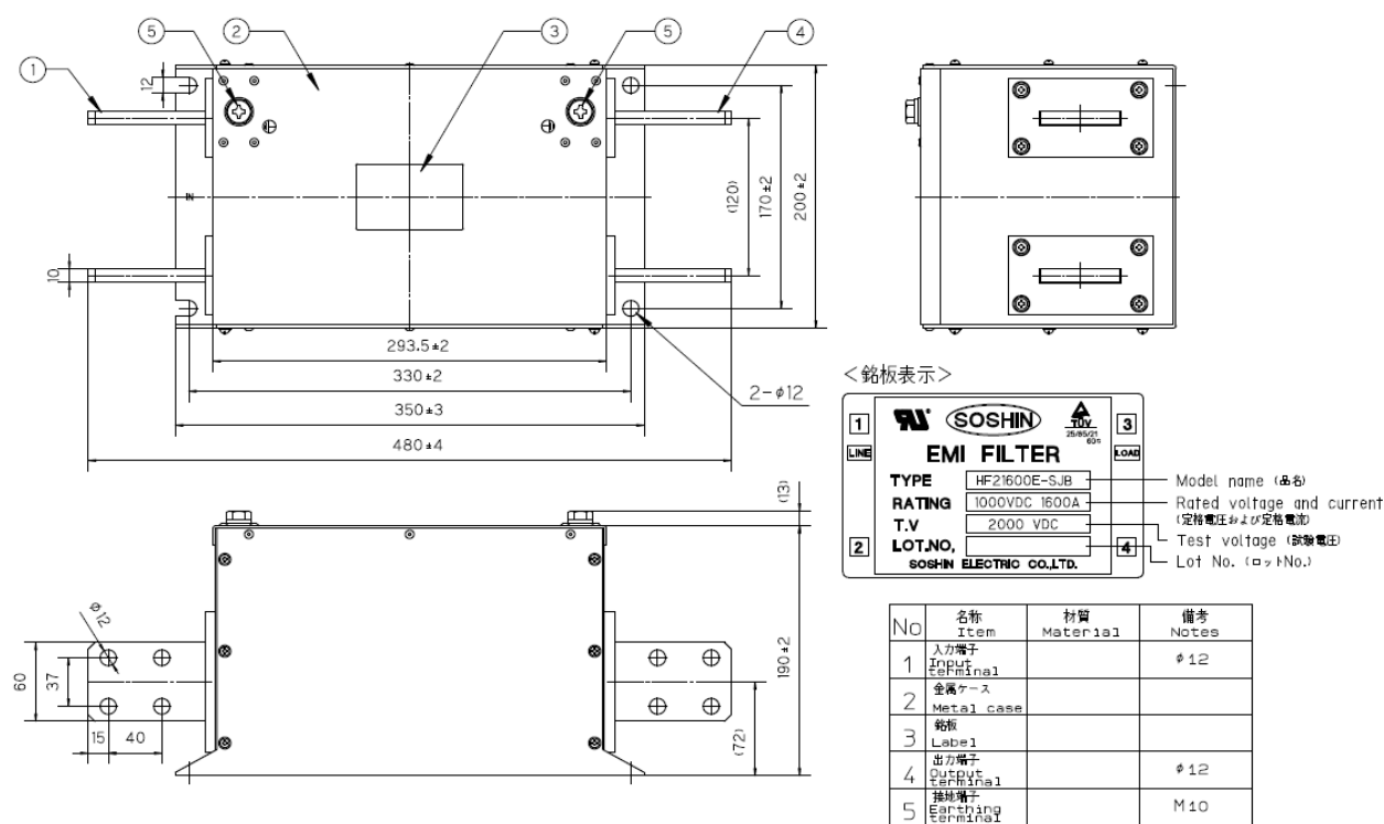
fig.4 (1600A)
