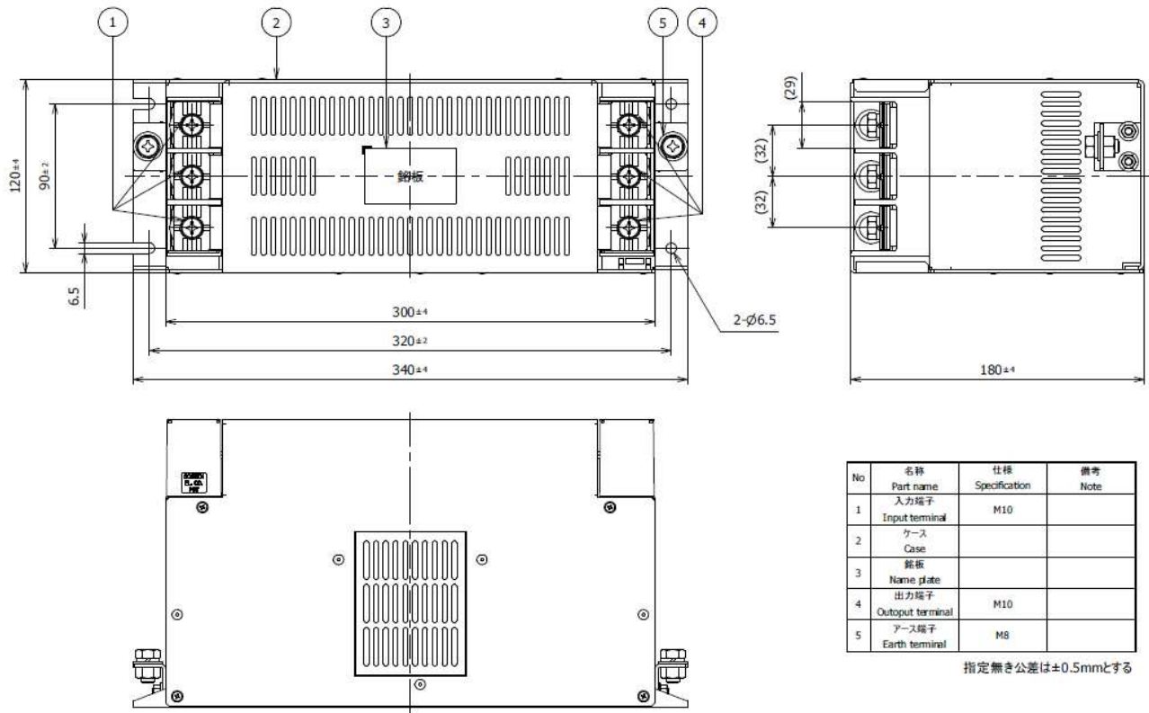
fig. 4 (200A~300A)
