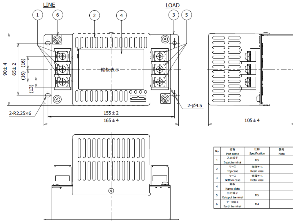
fig.2 (80A, 100A)
